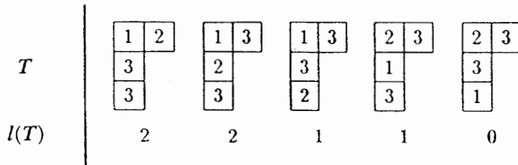
FIGURE 6. \lambda = (2, 1, 1) , \mu = (1, 1, 2) .
