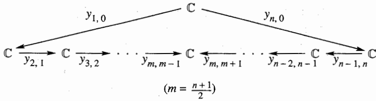
FIGURE 2. \Sigma .
