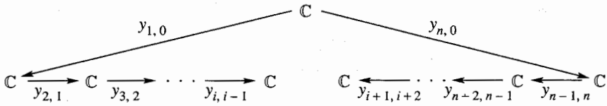
FIGURE 1. p_i .
